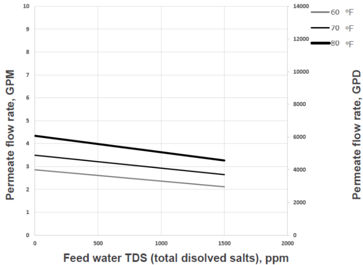
Figure 2.4 CROS4591 flow rate chart with TW30 PRO-4040 membranes
