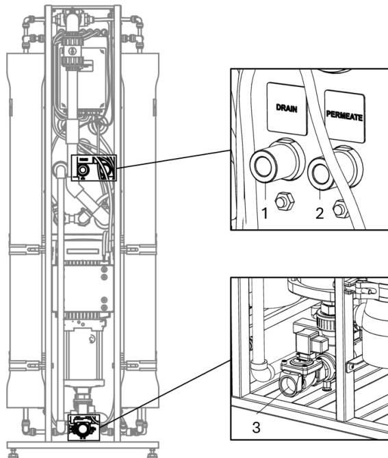
Figure 2.1 CROS4591 system water piping connection ports
