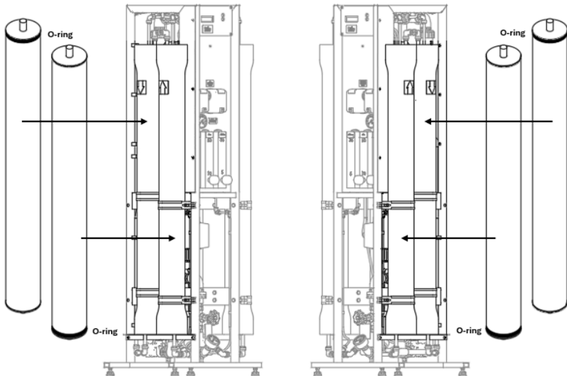
Figure 3.3 Correct position of the installed membrane
