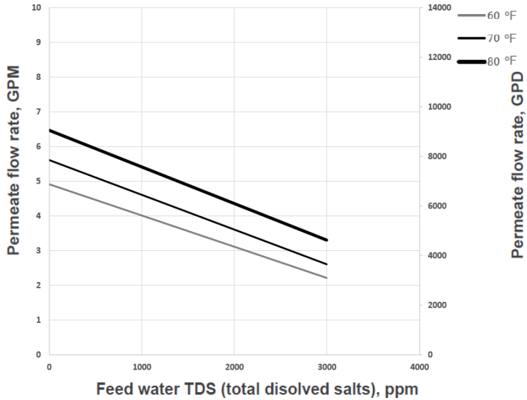
Figure 2.3 CROS4591 flow rate chart with XLE PRO-4040 membranes
